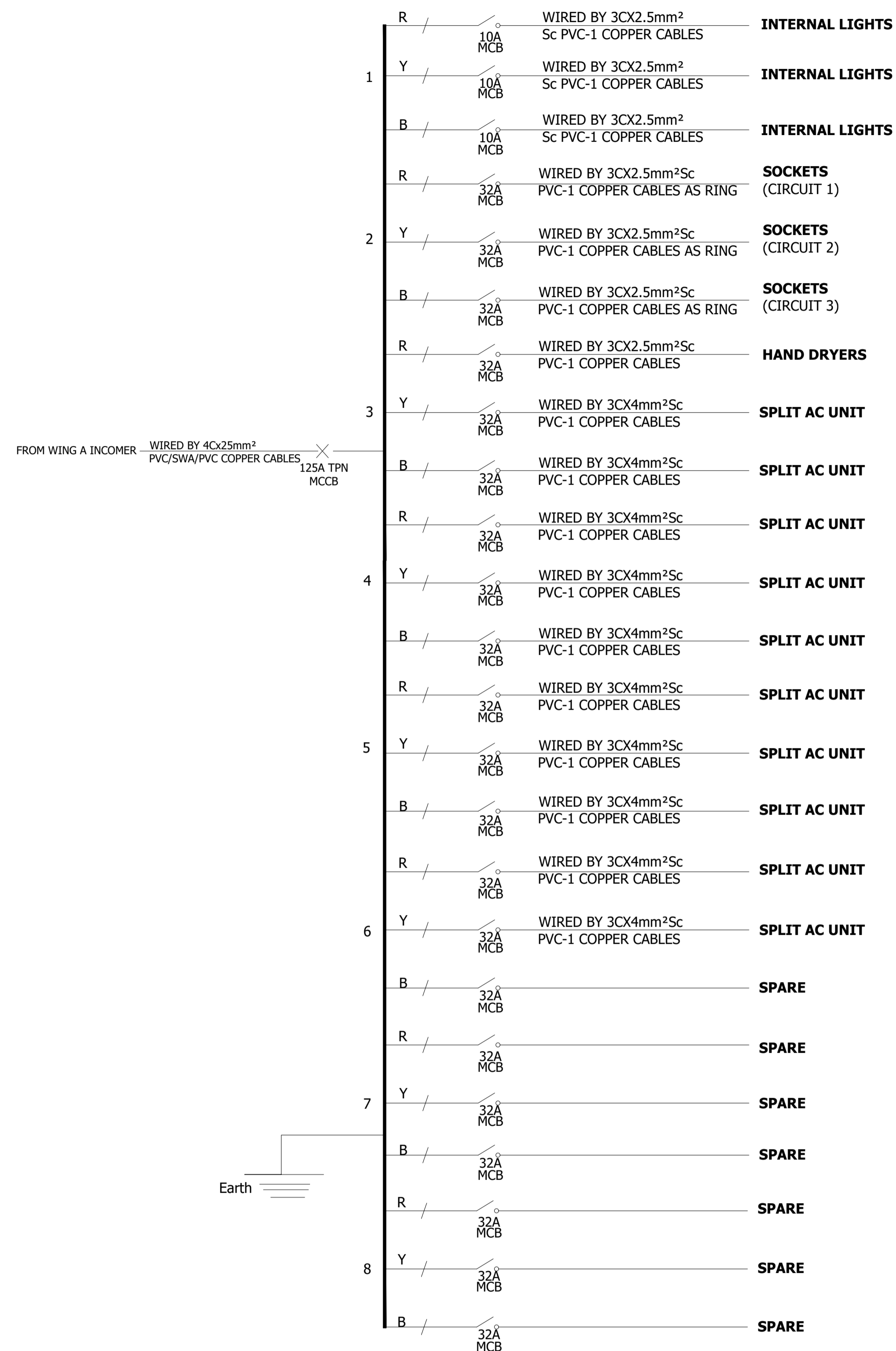
125A, 8-WAY TPN MCCB DISTRIBUTION BOARD (DB-6) RECESSED IN WALL IN DUCT ON THIRD FLOOR (WING B)
