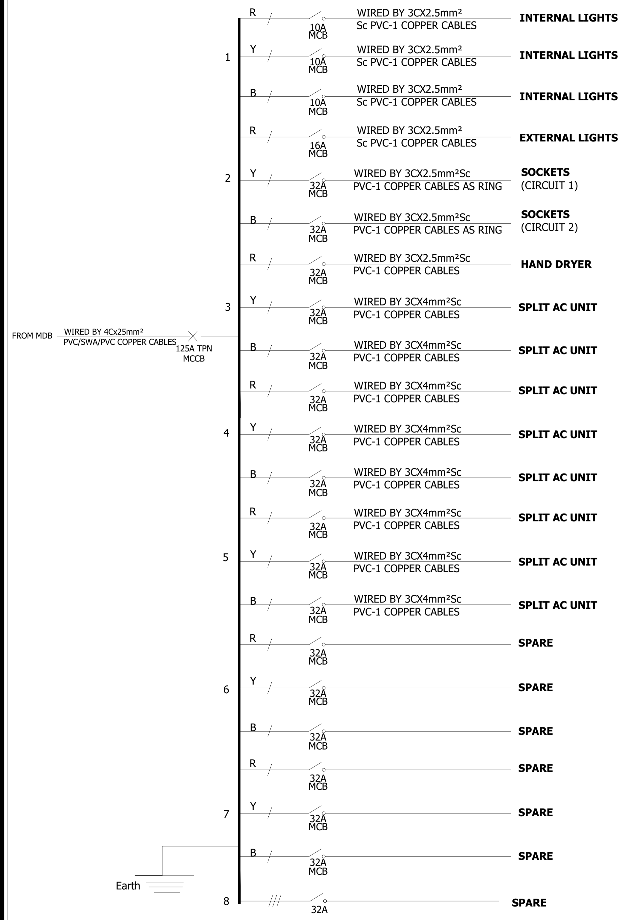
125A, 8-WAY TPN MCCB DISTRIBUTION BOARD (DB-1) RECESSED IN WALL IN DUCT ON GROUND FLOOR
