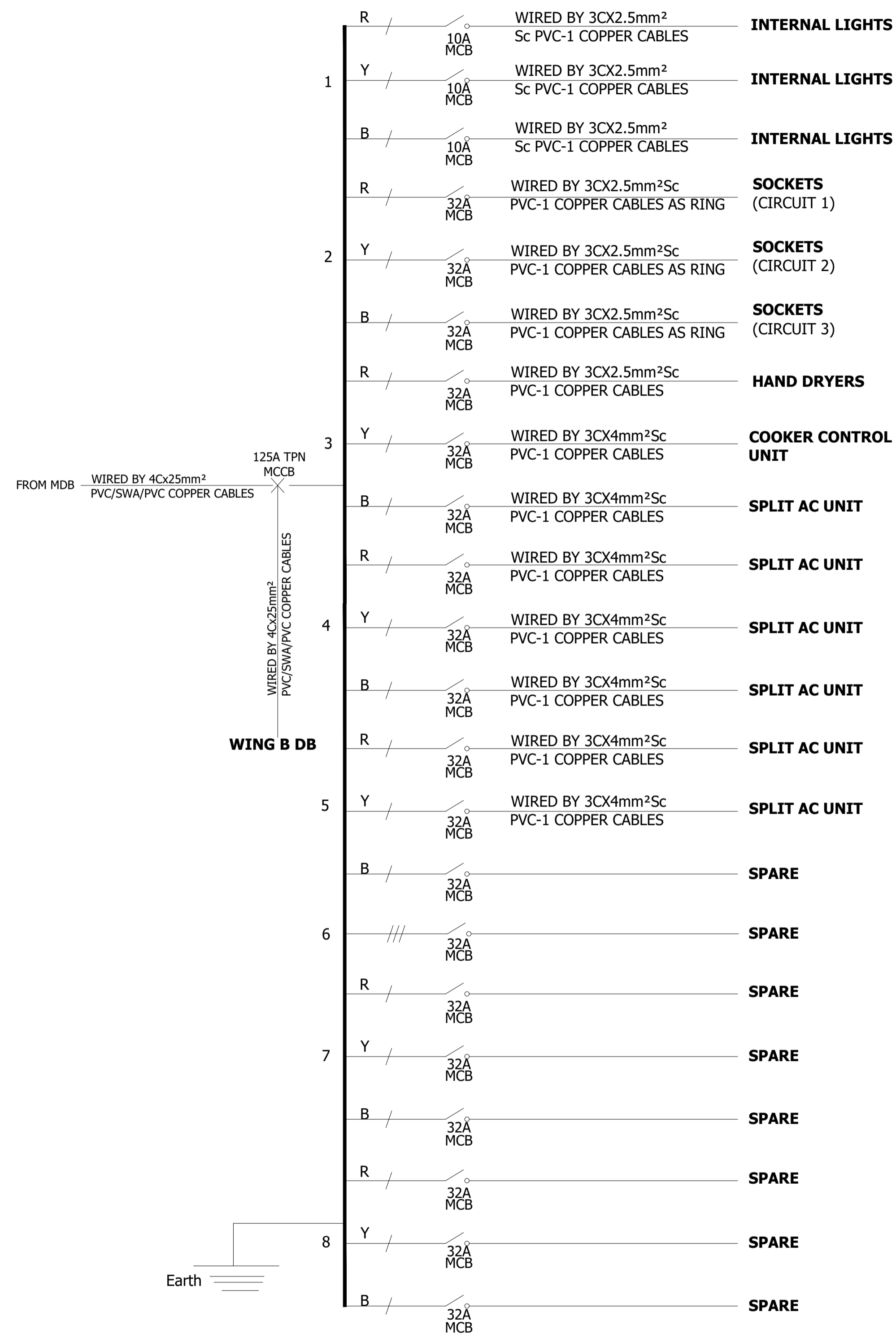
125A, 8-WAY TPN MCCB DISTRIBUTION BOARD (DB-5) RECESSED IN WALL IN DUCT ON THIRD FLOOR (WING A)
