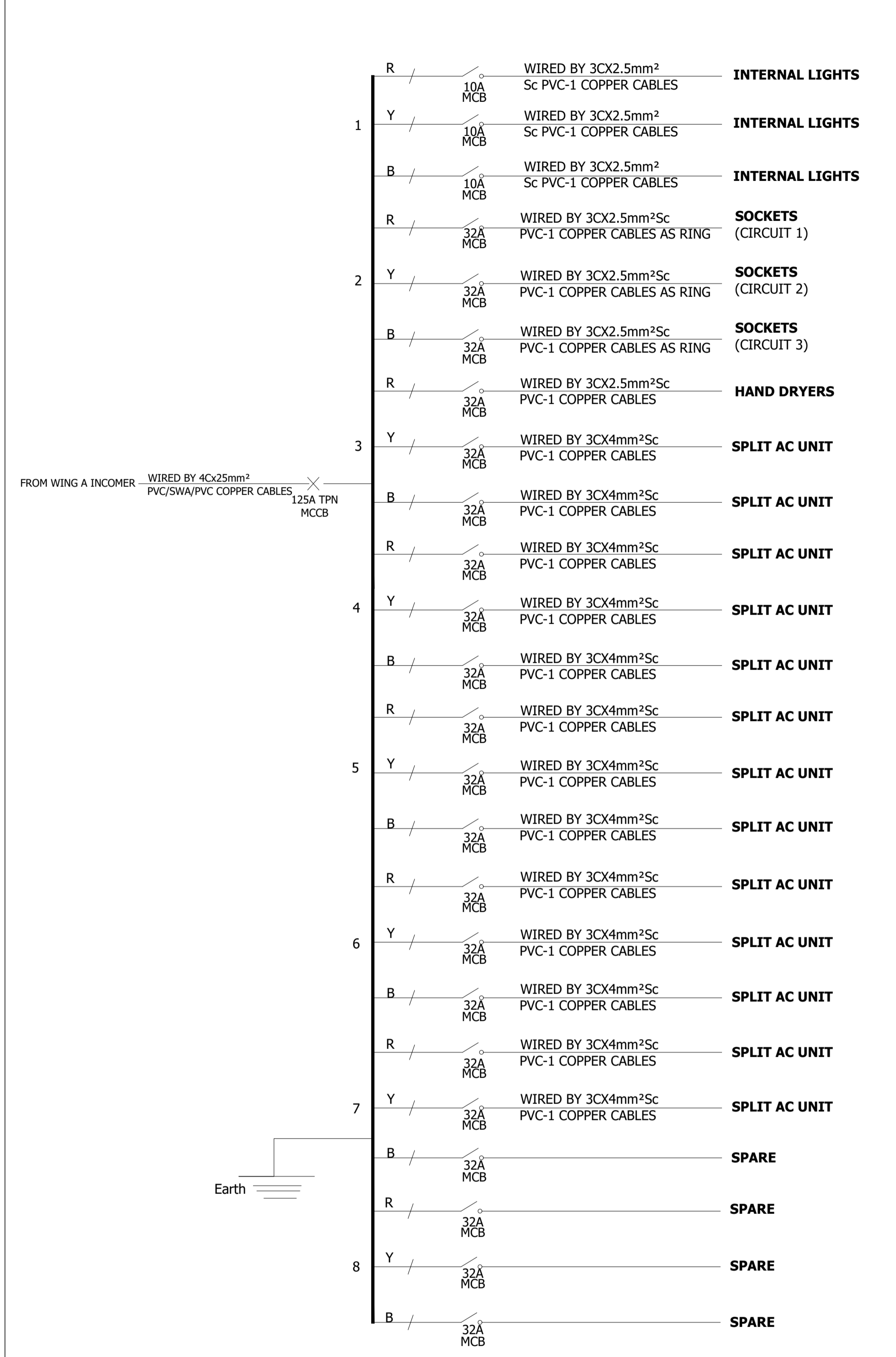
125A, 8-WAY TPN MCCB DISTRIBUTION BOARD (DB-4) RECESSED IN WALL IN DUCT ON SECOND FLOOR (WING B)
