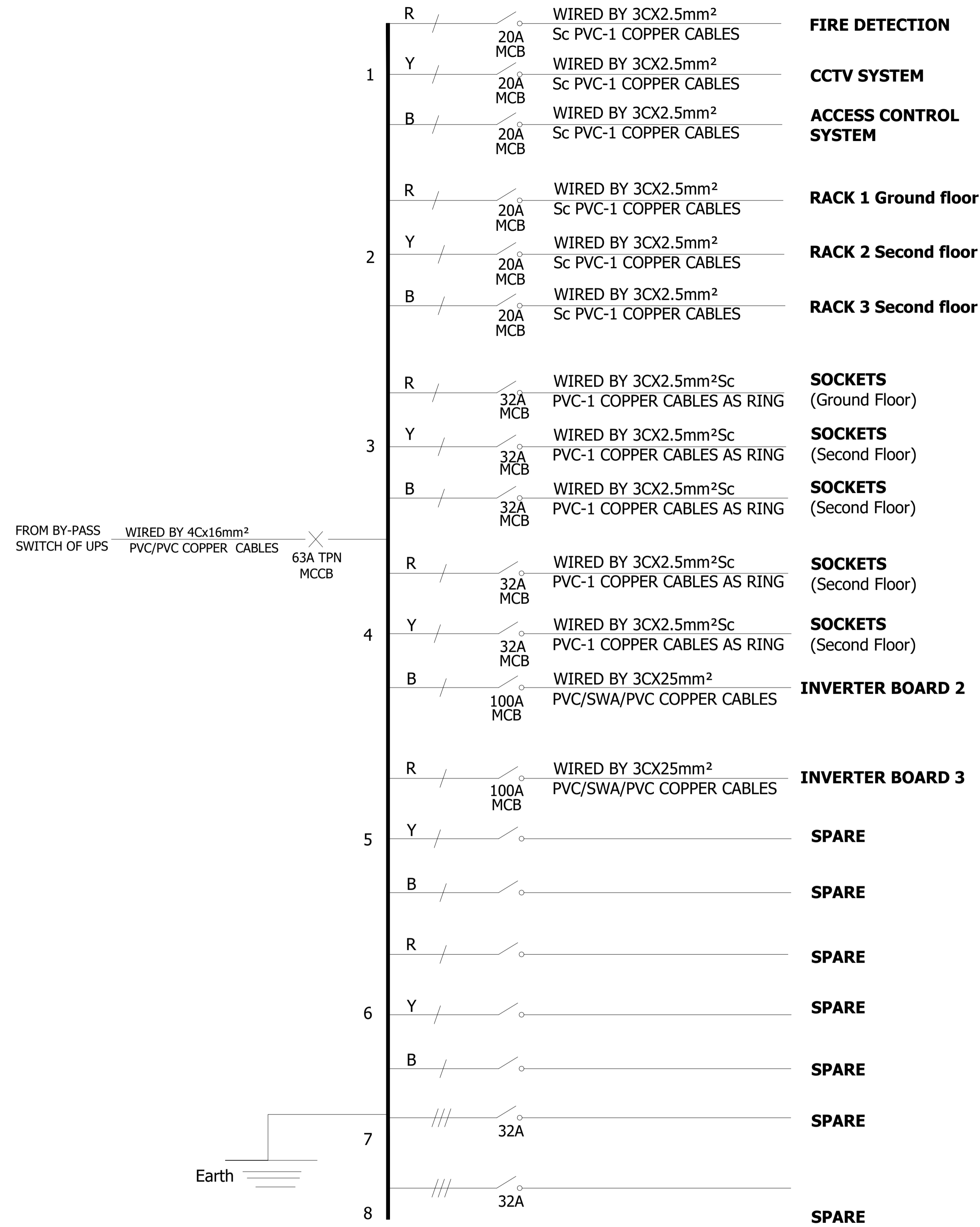
63A, 8-WAY TPN MCCB UPS DISTRIBUTION BOARD (UPS DB-1) RECESSED IN WALL AS CRABTREE, HAGER OR EQUAL APPROVED ON SECOND FLOOR SERVER ROOM
